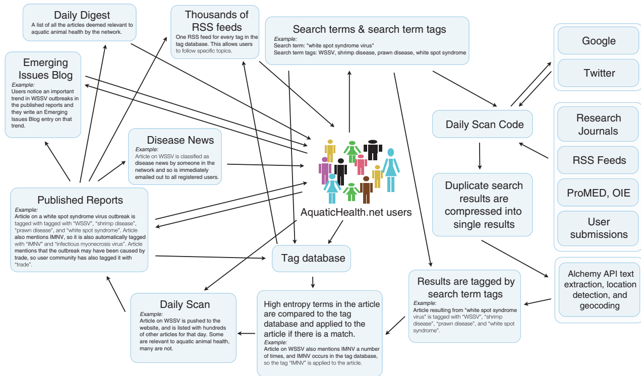
Figure 1 AquaticHealth.net's information flow.
